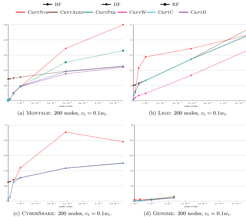
Figure 7: Impact of the checkpointing strategy. For each checkpointing strategy, we plot the best linearization strategy.
