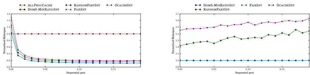
Figure 25: Impact of sequential fraction with RANDOM.
