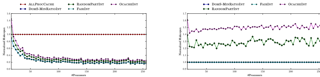
Figure 22: Impact of the number of processors with RANDOM.
