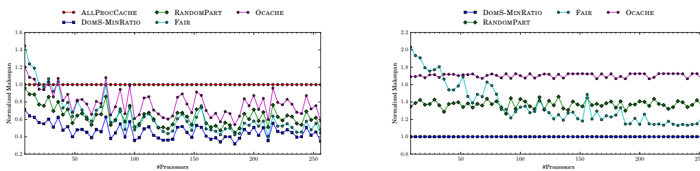
Figure 12: Impact of the number of processors with NPB-6.
