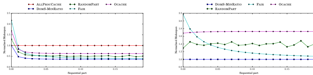
Figure 15: Impact of sequential fraction of work with NPB-6.
