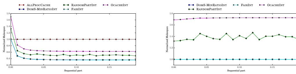
Figure 26: Impact of sequential fraction with NPB-6.
