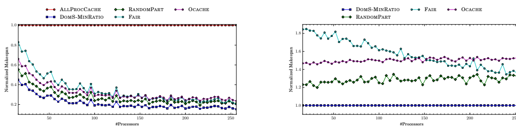
Figure 13: Impact of the number of processors with RANDOM and 16 applications.
