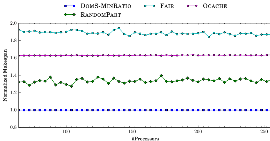
Figure 11: Impact of the number of processors with NPB-SYNTH and 64 applications.
