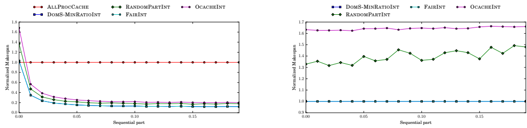
Figure 24: Impact of sequential fraction.
