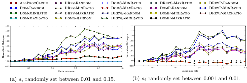
Figure 3: Impact of the cache miss ratio m_{40MB\mathcal{S}_s}^i with a 1GB cache and 16 applications.
