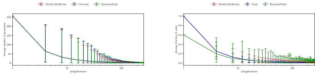
Figure 18: Processor and cache repartition with 256 processors with RANDOM.
