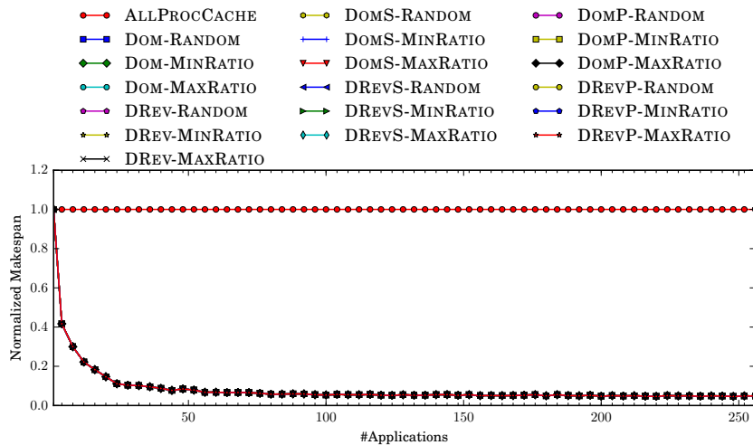
Figure 2: Comparison of all dominant partition heuristics on 256 processors.
