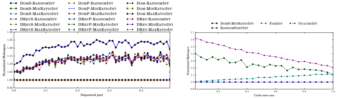
Figure 9: Impact of the sequential fraction and the cache miss rate.
