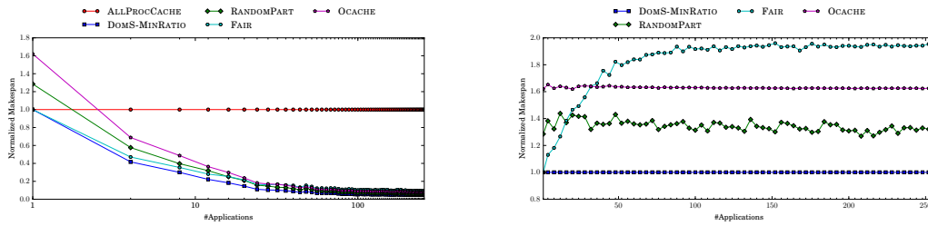
Figure 4: Impact of the number of applications.
