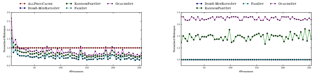
Figure 23: Impact of the number of processors with NPB-6.
