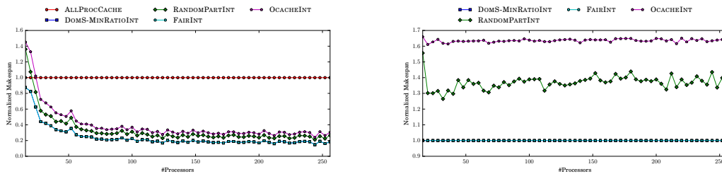
Figure 21: Impact of the number of processors with NPB-SYNTH.
