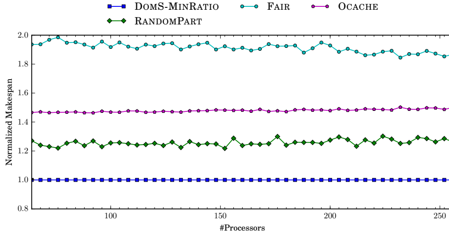
Figure 14: Impact of the number of processors with RANDOM and 64 applications (normalized with DOMS-MINRATIO).
