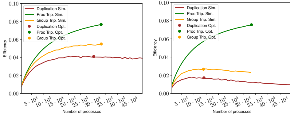
Figure 3: Impact of the number of processes on the efficiency with MTBE = 10^4 (left), MTBE = 10^3 (right), and c = 1800 , d = 0 , \alpha = 10^{-5} .
