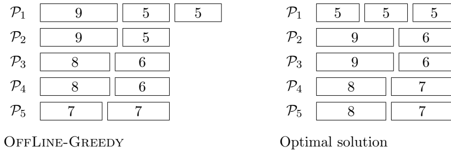
Figure 2: Tight instance for OFFLINE-GREEDY (with p = 5 ).
