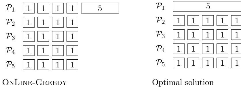
Figure 1: Tight instance for ONLINE-GREEDY (with p = 5 ).
