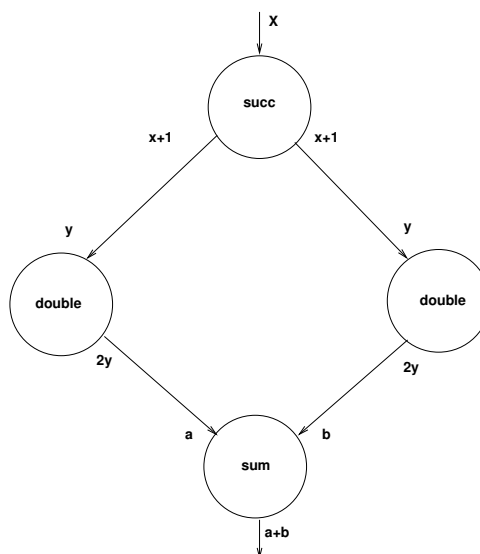
Figure 15.1: DAG example
