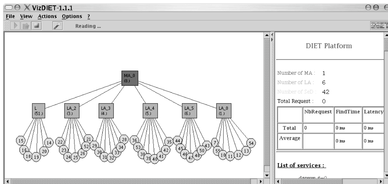
Figure 11.2: Snapshot of VizDIET.
