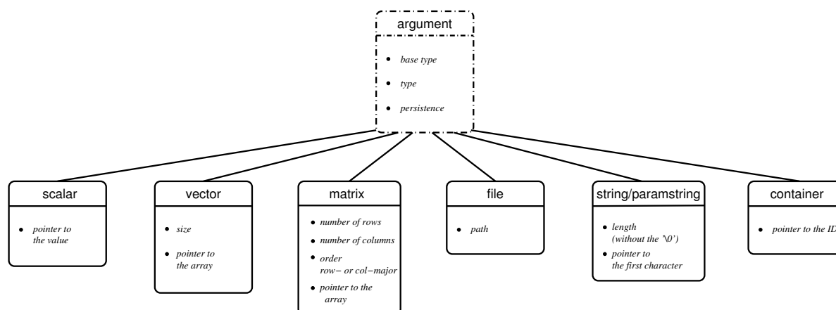
Figure 3.1: Argument/Data structure description.
