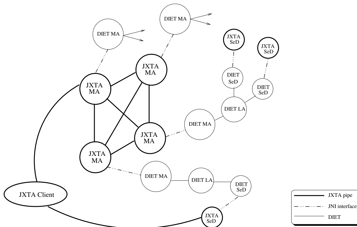
Figure 13.1: DIET_J architecture
