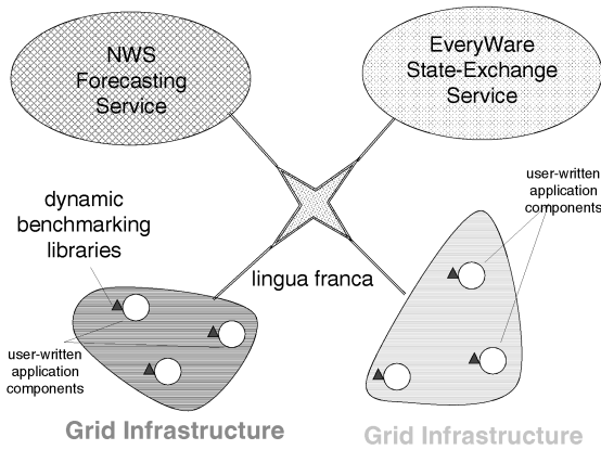
Fig. 1. EveryWare components.
