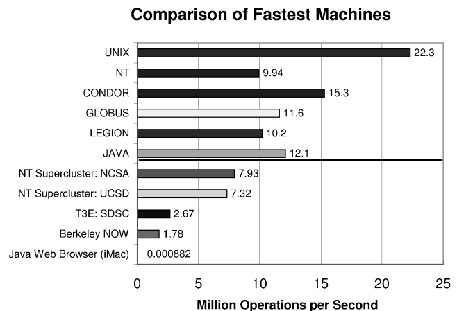
Fig. 10. Host speeds.
