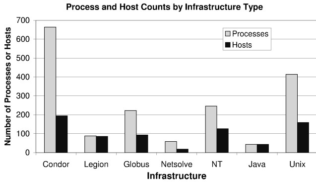
Fig. 8. Total host count by infrastructure.
