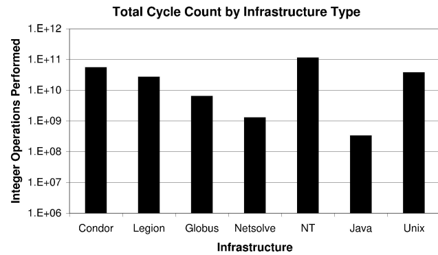
Fig. 7. Total cycle count by infrastructure.
