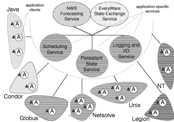
Fig. 2. EveryWare application structure.
