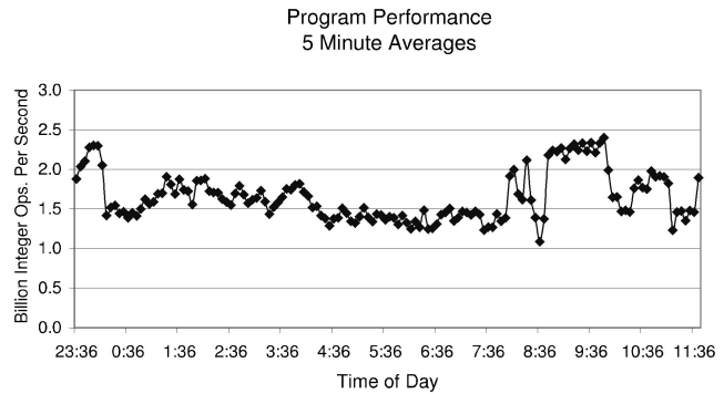
Fig. 3. Application speed.
