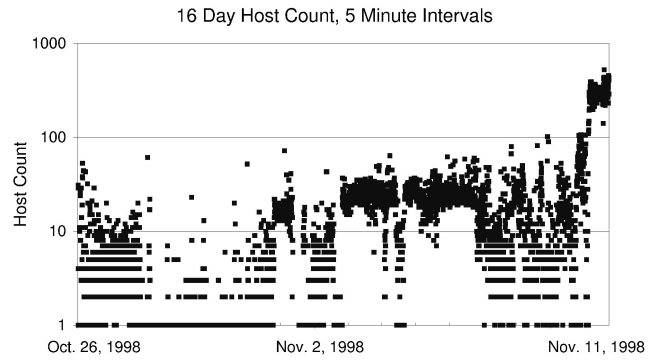
Fig. 9. Sixteen-day host counts.
