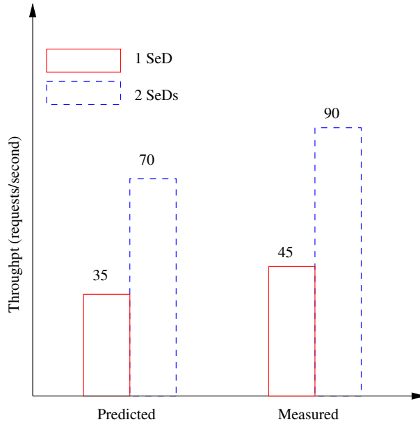
Fig. 5. Star hierarchies with one or two servers for DGEMM 200x200 requests. Comparison of predicted and measured maximum throughput.
