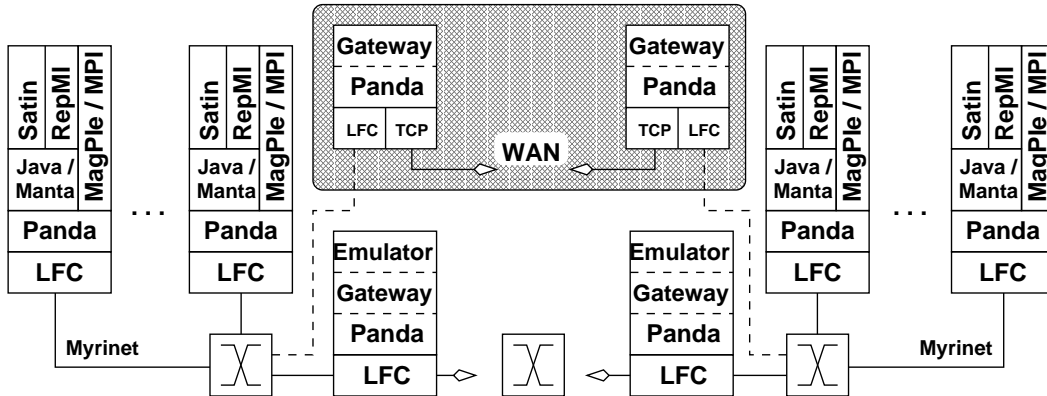
Fig. 2. Local and wide-area communication with Panda and the WAN emulator
