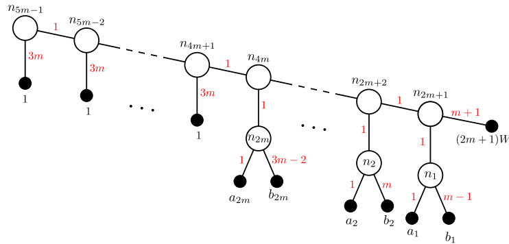
Figure 5: Instance \mathcal{I}_6 .
