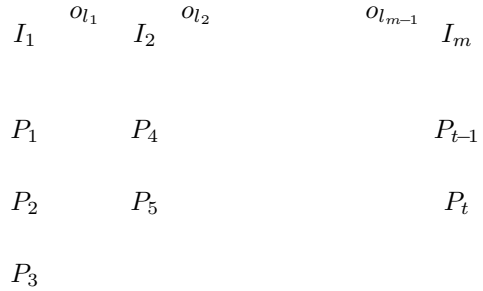
Figure 3. An example of interval mapping.
