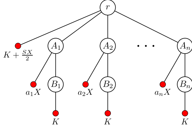
Figure 3: Illustration of the NP-completeness proof.
