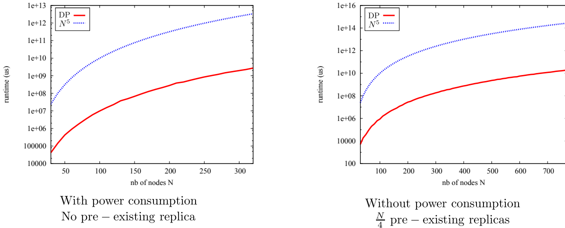
Figure 12: Running time of the DP algorithm.
