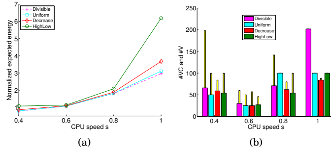
Fig. 12. Performance comparison of the ENERGY-VC+V algorithm and the periodic checkpointing and verification algorithm for divisible load application.
