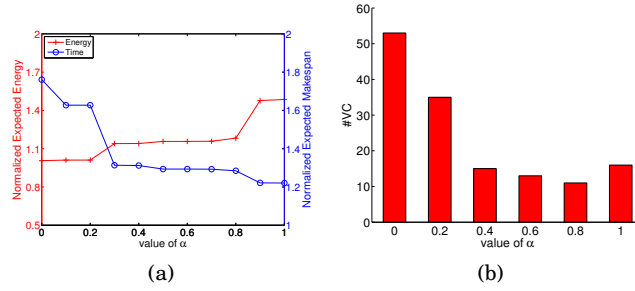
Fig. 19. Performance of the TIMEENERGY-VC+V algorithm with different values of \alpha in the MULTISPEED scenario.
