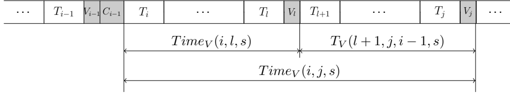
Fig. 5. Illustration of the dynamic programming formulation for Time_V(i, j, s) .
