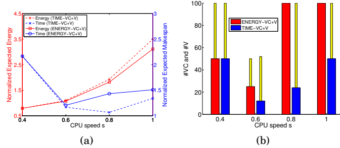
Fig. 13. Performance of the ENERGY-VC+V and TIME-VC+V algorithms with different CPU speeds.
