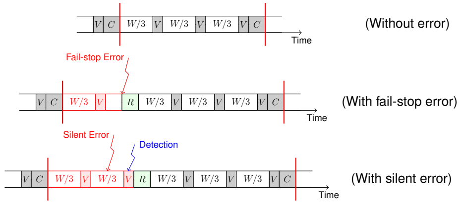
Fig. 2. The VC+V pattern with k = 3 chunks executed at unit speed s = 1 . The first figure shows the execution of a pattern without any error. The second figure shows that the execution is stopped immediately when a fail-stop error strikes anywhere in the pattern. The third figure shows that the execution continues after a silent error strikes and it is detected by an additional verification before the end of the pattern. In both cases, the pattern is re-executed after a recovery.
