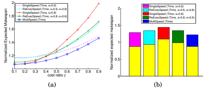
Fig. 16. Performance comparison of the TIME-VC+V algorithms in MULTISPEED, REEXECSPED and SINGLESPEED scenarios for n = 100 tasks under HighLow distribution. In (b), the cost ratio is fixed at \gamma = 0.6 , and the yellow part at the bottom of each bar represents the expected execution time for the large tasks.
