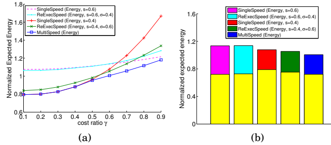
Fig. 17. Performance comparison of the ENERGY-VC+V algorithms in MULTISPEED, REEXECSPED and SINGLESPEED scenarios for n = 100 tasks with HighLow distribution. In (b), the cost ratio is fixed at \gamma = 0.6 , and the yellow part at the bottom of each bar represents the expected energy consumption for the large tasks.
