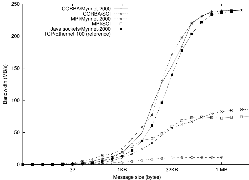
Fig. 4. CORBA and MPI bandwidth on top of PadicoTM
